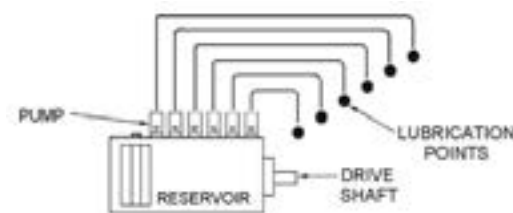
PUMP-TO-POINT SYSTEM
